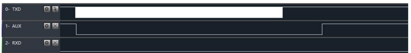
Timing sequence chart of AUX when MCU receives serial data till MCU starts RF transmission
